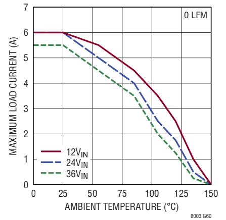
Derating, H-Grade, V_{OUT} = 5\text{V} , BIAS = 5V, DC2416A Demo Board
