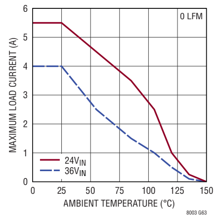
Derating, H-Grade, V_{OUT} = 15\text{V} , BIAS = 5V, DC2416A Demo Board
