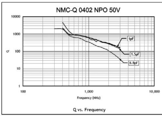
Link 0402 Q vs. Frequency
