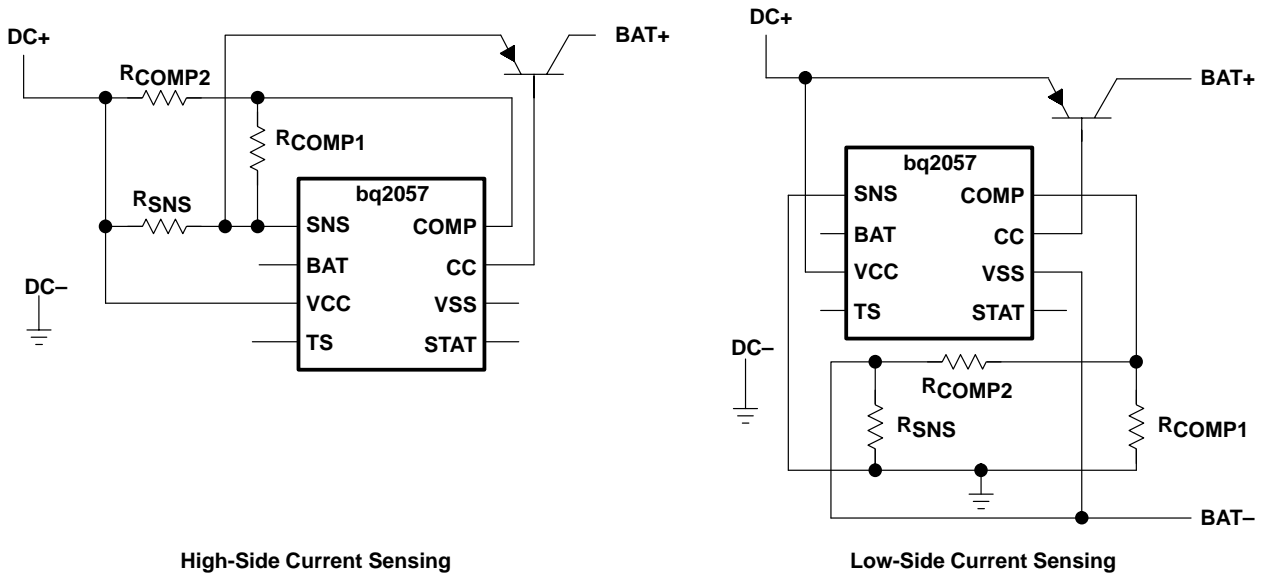
Figure 13. AutoComp Circuits
