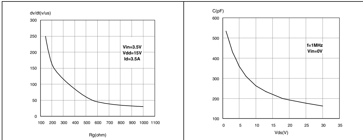
Figure 23. Output characteristics
