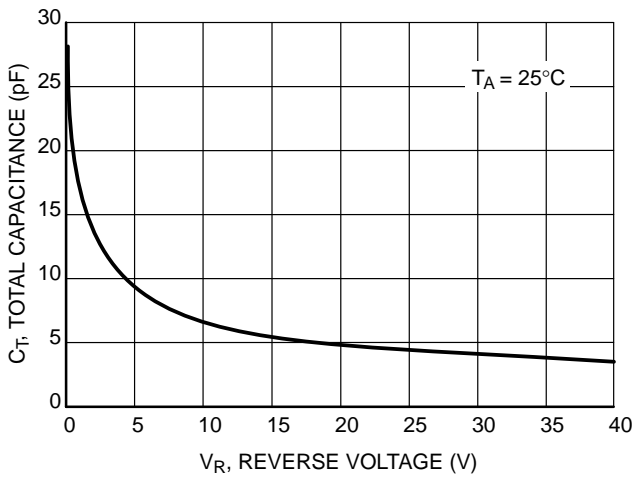
Figure 4. Total Capacitance
