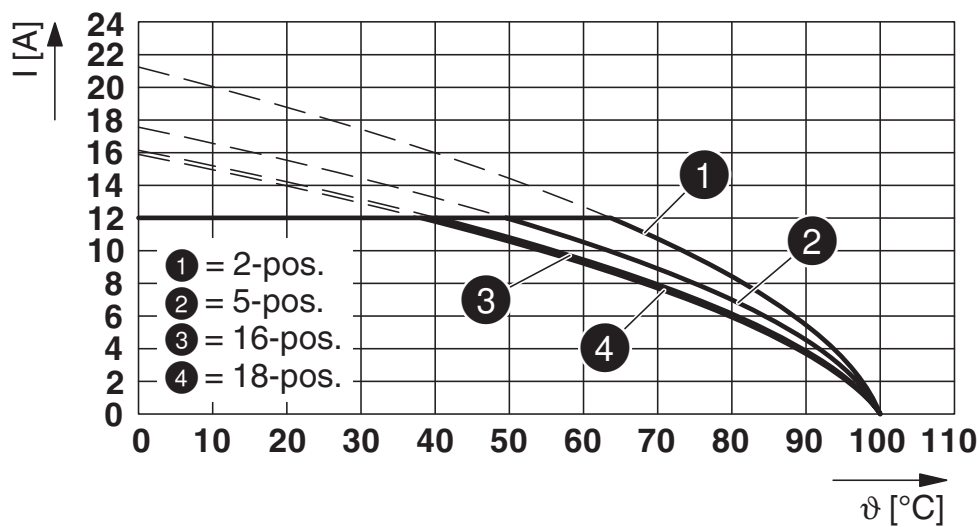
Type: FKCV(W/R) 2,5/...-ST with MSTBV 2,5/...-G
