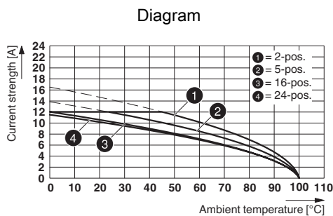
Type: SMSTB 2,5/...-ST with MSTBV 2,5/...-G
