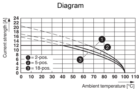
Type: FKCS 2,5/...-ST with MSTBV 2,5/...-G
