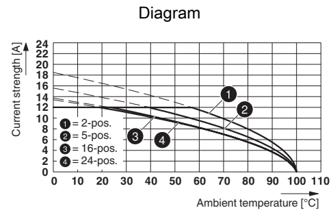
Type: FRONT-MSTB 2,5/...-ST with MSTBV 2,5/...-G
