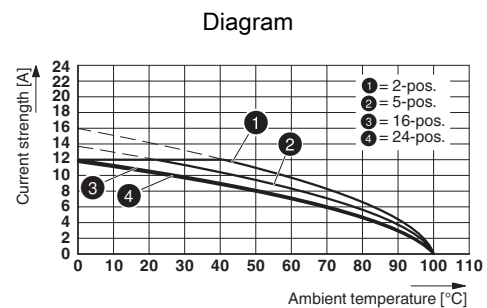
Type: MVSTB(R/W) 2,5/...-ST with MSTBV 2,5/...-G
