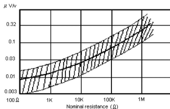
Current Noise
