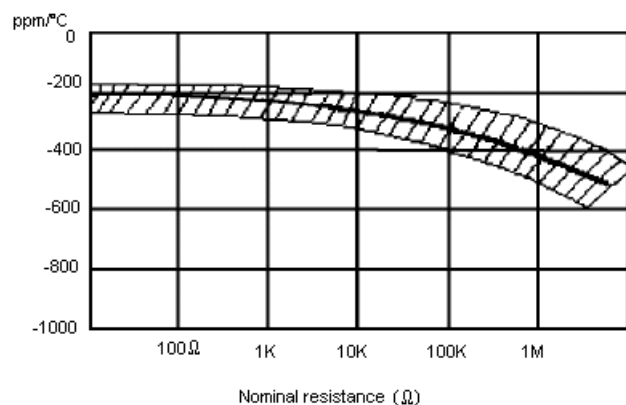
Temperature Coefficient
