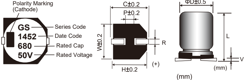
Fig.2 \text{ØD}\geq 12.5\text{mm}
