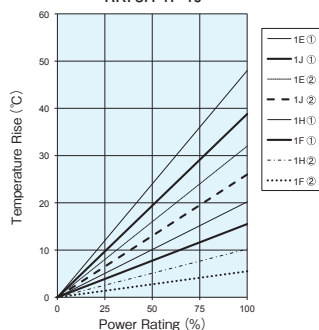
RK73H 1F-1J
