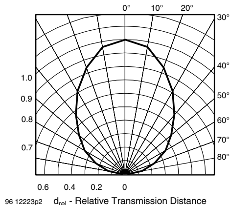
Fig. 12 - Horizontal Directivity
