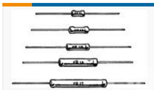
TE Part #8-2176091-9 RP 2A 0.25W 499R 0.1% 25PPM 1K RL
