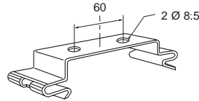
Mounting bracket clip V014: stainless steel
