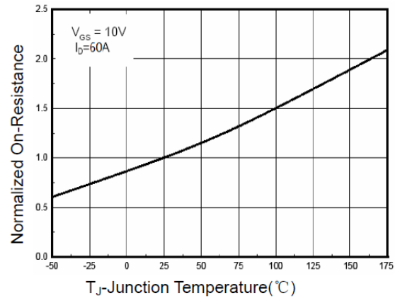
Figure 4 Rdson-Junction Temperature
