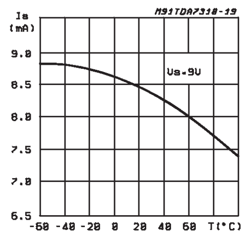
Figure 14: Supply Current vs. Temperature
