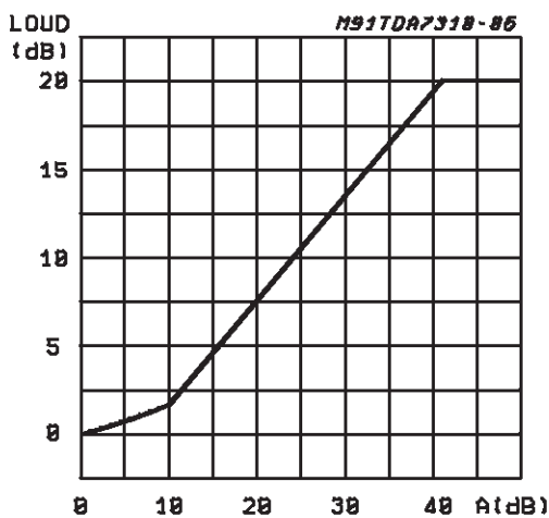
Figure 1: Loudness vs. Volume Attenuation
