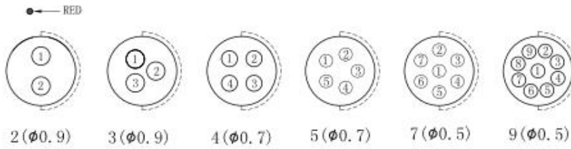
CONNECTOR SOLDER CUP VIEW
