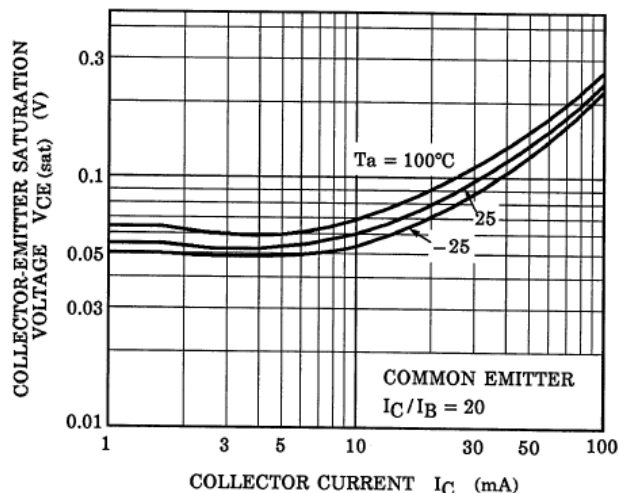
Fig. 10.24 RN1406 V_{CE(sat)}-I_C
