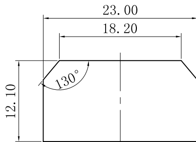
PANEL CUT-OUT
