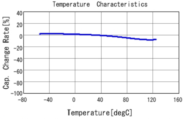
GRM033R71A332KA01 C-Temp. capchange, DC0.0V, AC1.C
