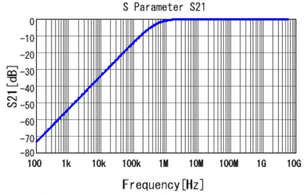
GRM033R71A332KA01 S21 DC0V, 25degC
