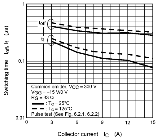
Fig. 8.10 t_{off}, t_r - I_C
