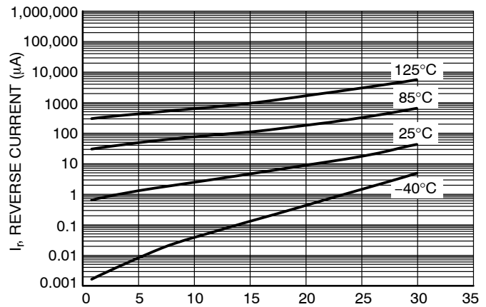
V_R , REVERSE VOLTAGE (V) Figure 2. Leakage Current
