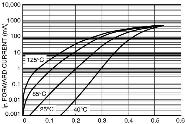
V_F FORWARD VOLTAGE (V) Figure 1. Forward Voltage
