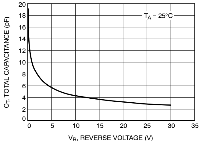
V_R , REVERSE VOLTAGE (V) Figure 3. Total Capacitance
