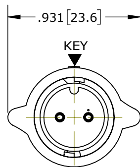
MATING FACE ASSY: W6280-2SG-P-5XX SHOWN
