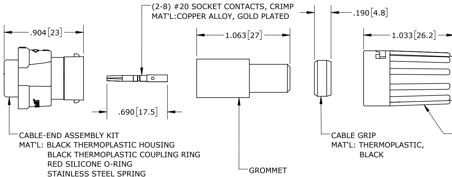
SHOWN ASSEMBLED KIT ASSY: W6280-2SG-P-5XX SHOWN
