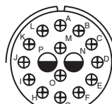
24-7 Service Rating A Number of Contacts 2 14 Contact Size 12 16
