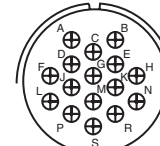
24-5 Service Rating A Number of Contacts 16 Contact Size 16
