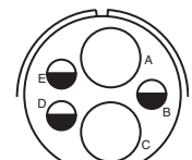
24-12 Service Rating A Number of Contacts 2 3 Contact Size 4 12
