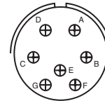
22-33 Service Rating A, B, C, D = D; E, F, G = A Number of Contacts 7 Contact Size 16
