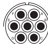
24-10 Service Rating A Number of Contacts 7 Contact Size 8
