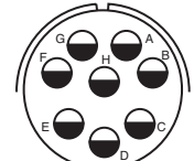
24-6 Service Rating A, G, H = D; Bal. = A Number of Contacts 8 Contact Size 12
