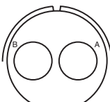
24-9 Service Rating A Number of Contacts 2 Contact Size 4
