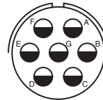
22-28 Service Rating A Number of Contacts 7 Contact Size 12
