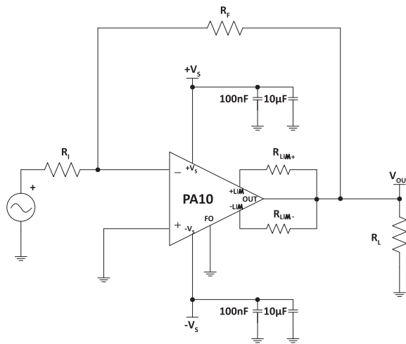
Figure 2: Typical Connection
