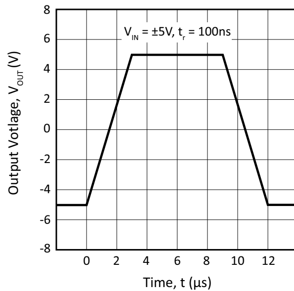
Figure 11: Pulse Response
