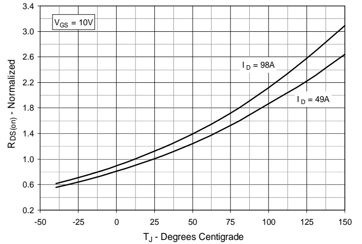
Fig. 4. R_{DS(on)} Normalized to I_D = 49A Value vs. Junction Temperature
