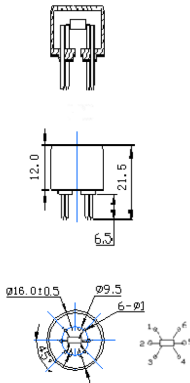
Fig1.Sensor Structure
