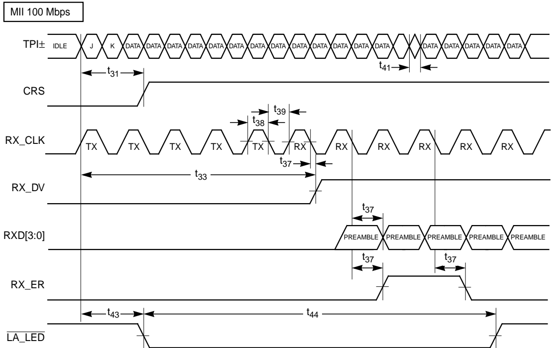
Figure 19 Receive Timing, Start of Packet - 100 Mbps
