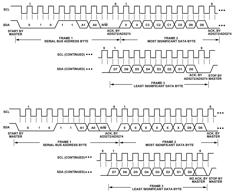
Figure 45. Read Command
