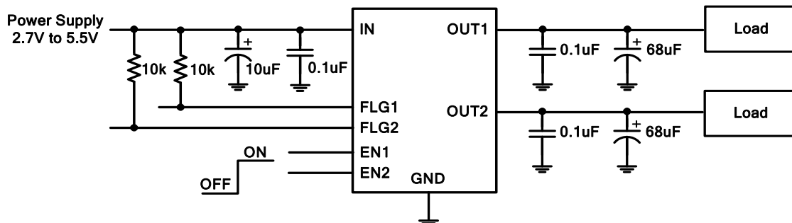
AP2172 Enable Active High
