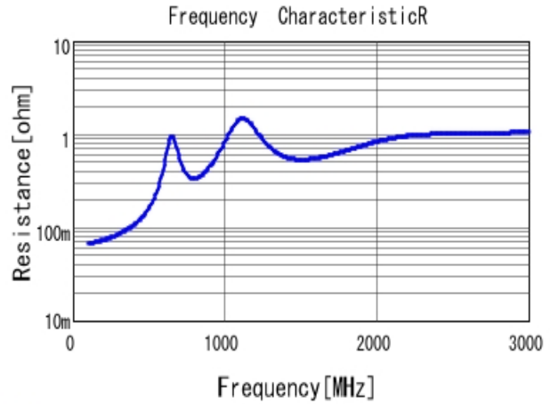
■ GRM31A5C2J561JW01 R DC0V, 25degC
