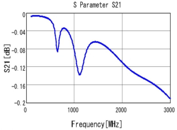
■ GRM31A5C2J561JW01 S21 DCOV, 25degC
