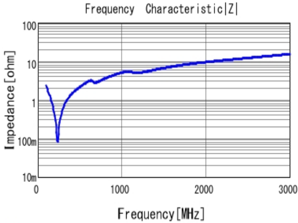
■ GRM31A5C2J561JW01 |Z| DC0V, 25degC
