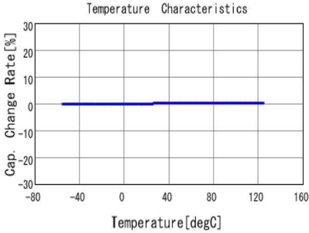
■ GRM31A5C2J561JW01 C-Temp. capchange, DCOV, AC1Vrms
