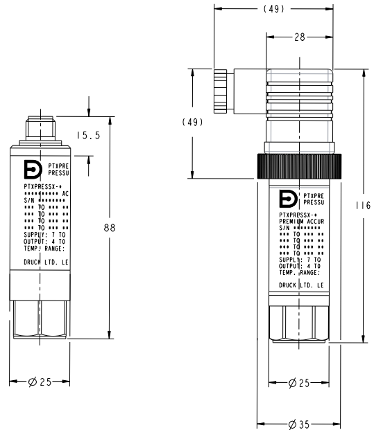
M12 x 1 4-pin Construction
