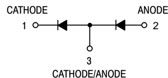
BAV99RWT1 SC-70, CASE 419, STYLE 10
