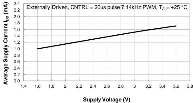
Average Supply Current (CNTRL = PWM) vs Supply Voltage
