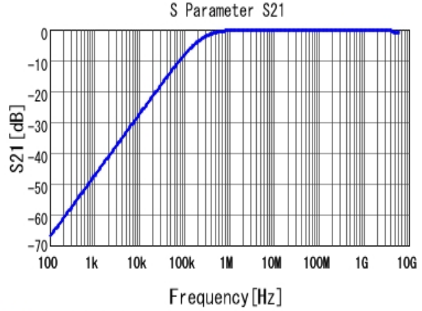
■ GRM219R72A682KA01 S21 DCOV, 25degC
