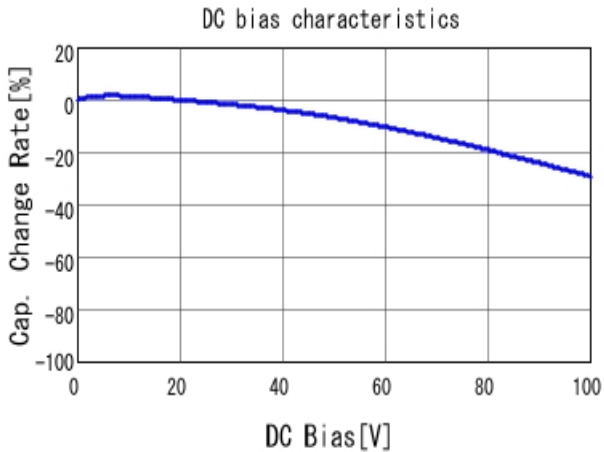
■ GRM219R72A682KA01 C-DC bias capchange, 25.0degC, AC1.
