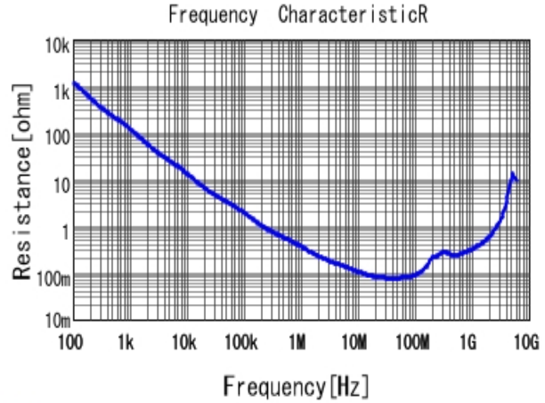
■ GRM219R72A682KA01 R DCOV, 25degC
