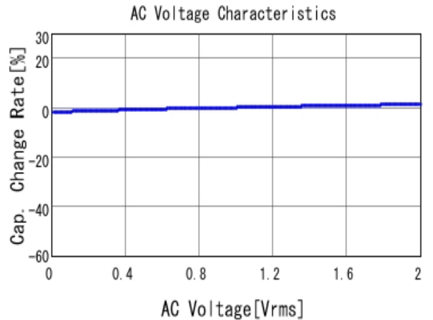
■ GRM219R72A682KA01 C-AC Voltage capchange, DCOV, 25.0d
