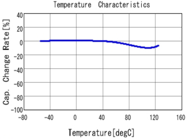
■ GRM219R72A682KA01 C-Temp. capchange, DCO. 0V, AC1.0Vrm
