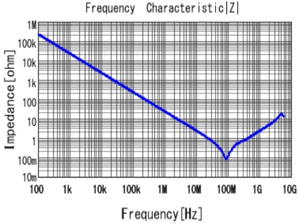
■ GRM219R72A682KA01 |Z| DCOV, 25degC
