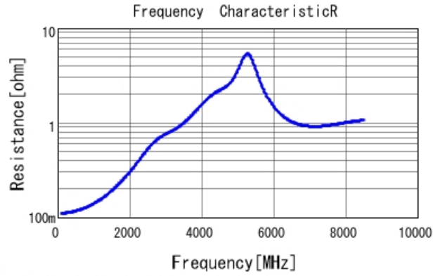
■ GRM0335C1H750JA01 R DCOV, 25degC
