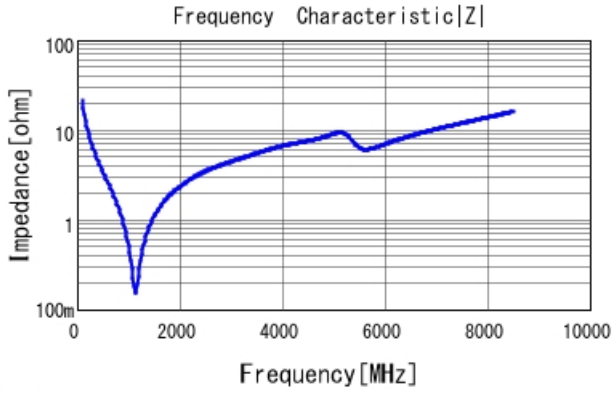
■ GRM0335C1H750JA01 |Z| DCOV, 25degC
