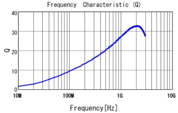
■ LQP03TN10NJ02 Q
