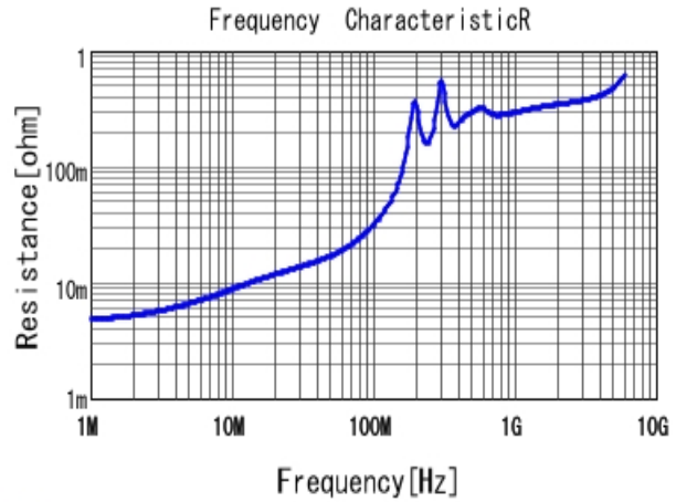
■ GRM2195C1H562JA01 R DCOV, 25degC
