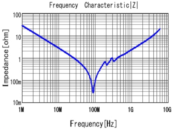
■ GRM2195C1H562JA01 |Z| DCOV, 25degC
