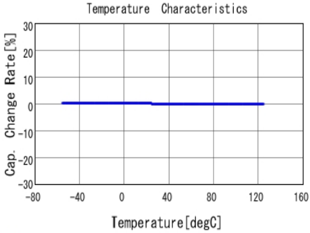
■ GRM2195C1H562JA01 C-Temp. capchange, DCOV, AC1Vrms
