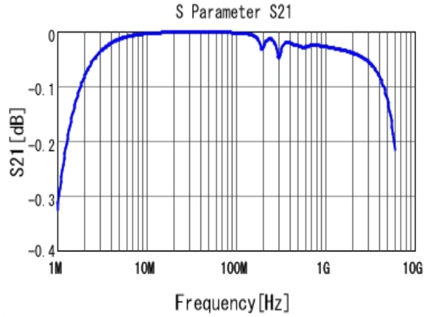
■ GRM2195C1H562JA01 S21 DCOV, 25degC
