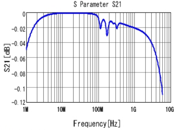
■ GRM2195C1H153JA01 S21 DCOV, 25degC
