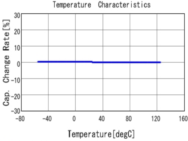
■ GRM2195C1H153JA01 C-Temp. capchange, DCOV, AC1Vrms
