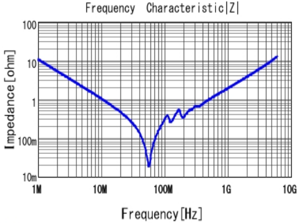
■ GRM2195C1H153JA01 |Z| DCOV, 25degC
