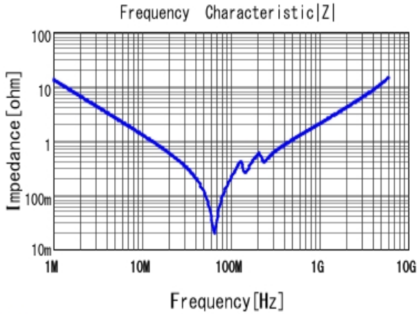
■ GRM2195C1H123JA01 |Z| DCOV, 25degC
