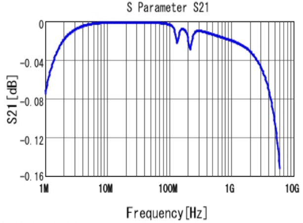
■ GRM2195C1H123JA01 S21 DCOV, 25degC
