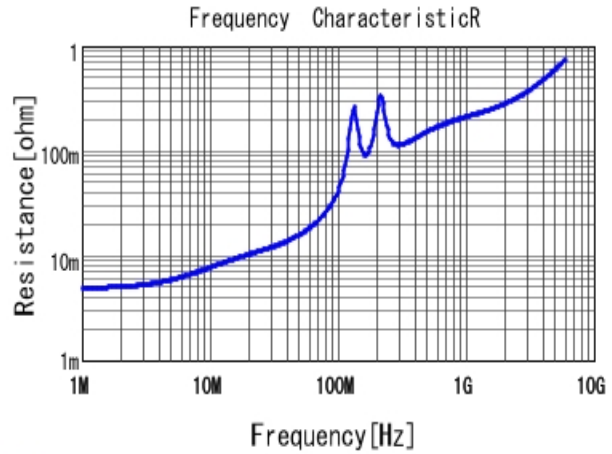
■ GRM2195C1H123JA01 R DCOV, 25degC
