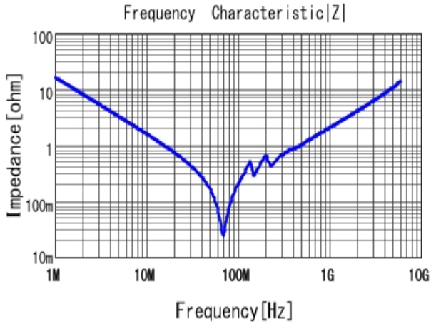
■ GRM2195C1H103JA01 |Z| DCOV, 25degC
