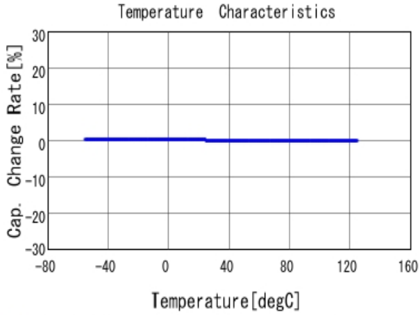
■ GRM2195C1H103JA01 C-Temp. capchange, DCOV, AC1Vrms
