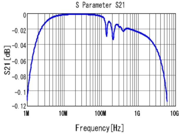
■ GRM2195C1H103JA01 S21 DCOV, 25degC
