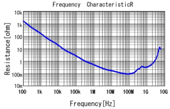
■ GRM216R71H472KA01 R DCOV, 25degC
