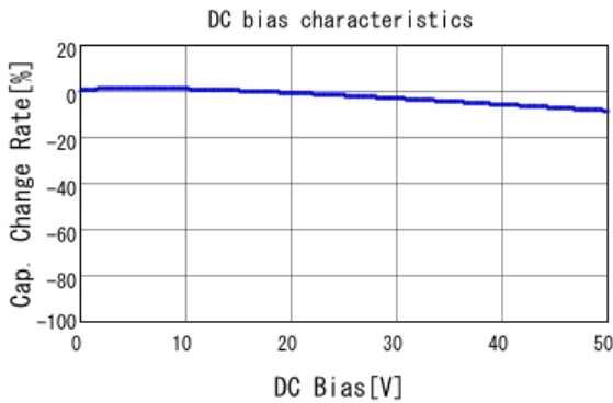
■ GRM216R71H472KA01 C-DC bias capchange, 25.0degC, AC1.
