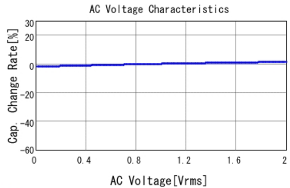
■ GRM216R71H472KA01 C-AC Voltage capchange, DCOV, 25.0d
