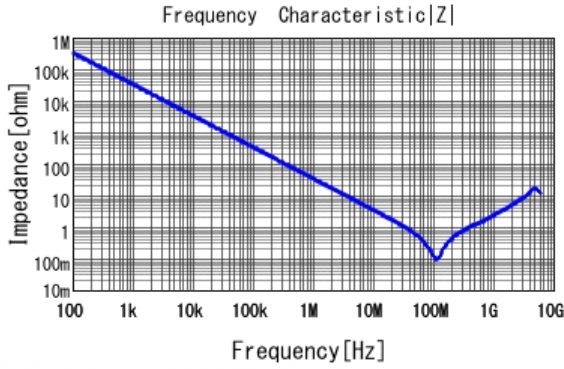
■ GRM216R71H472KA01 |Z| DCOV, 25degC
