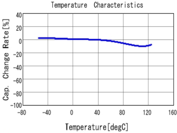
■ GRM216R71H223KA01 C-Temp. capchange, DCO. 0V, AC1.0V rm
