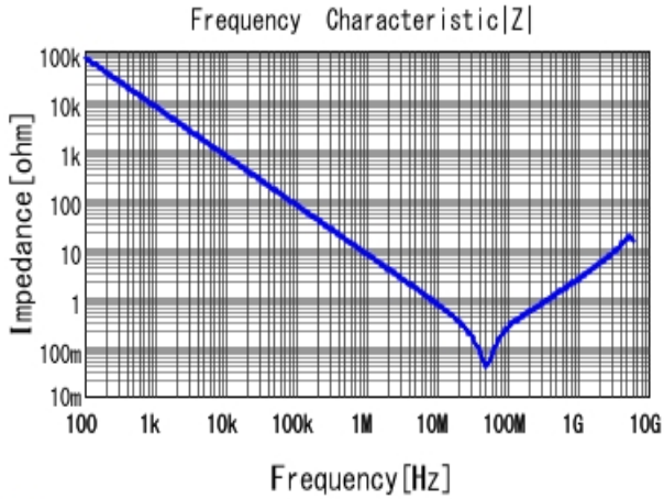
■ GRM216R71H223KA01 |Z| DCOV, 25degC
