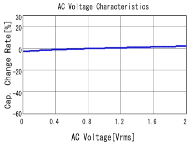
■ GRM216R71H223KA01 C-AC Voltage capchange, DCOV, 25.0d
