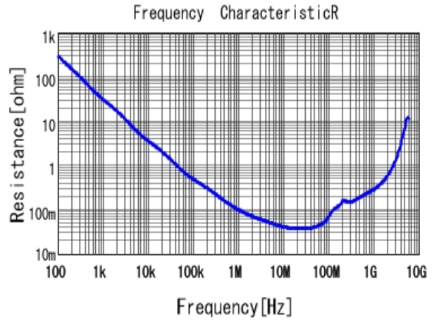
■ GRM216R71H223KA01 R DCOV, 25degC
