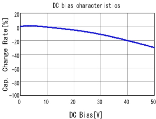
■ GRM216R71H223KA01 C-DC bias capchange, 25.0degC, AC1.
