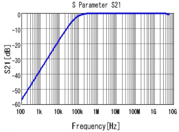
■ GRM216R71H223KA01 S21 DCOV, 25degC
