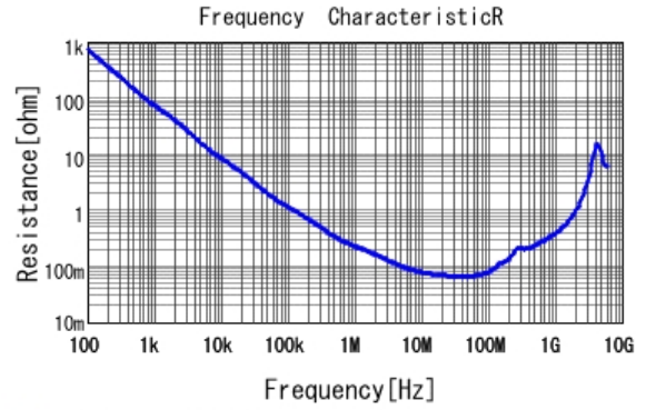
■ GRM216R71H103KA01 R DCOV, 25degC
