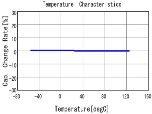
■ GRM2165C2A471JA01 C-Temp. capchange, DCOV, AC1Vrms
