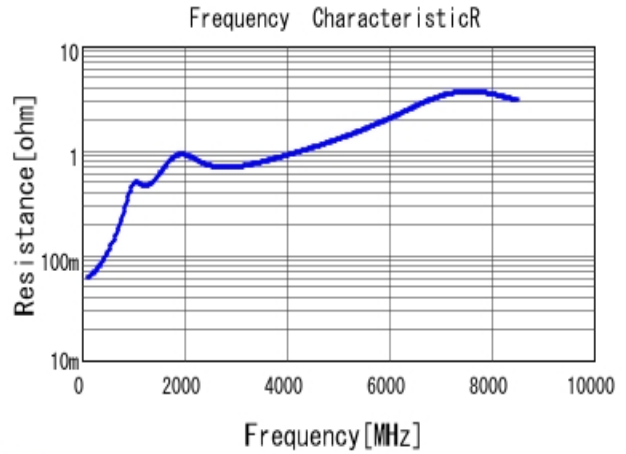
■ GRM2165C2A471JA01 R DC0V, 25degC
