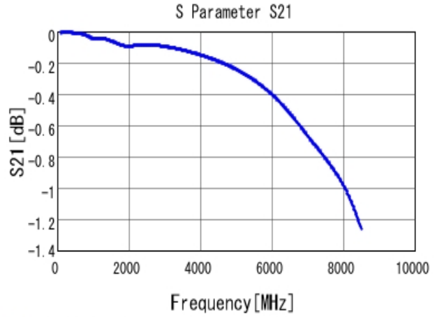
■ GRM2165C2A471JA01 S21 DCOV, 25degC
