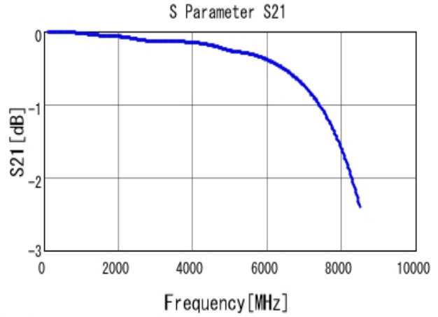
■ GRM2165C2A331JA01 S21 DCOV, 25degC
