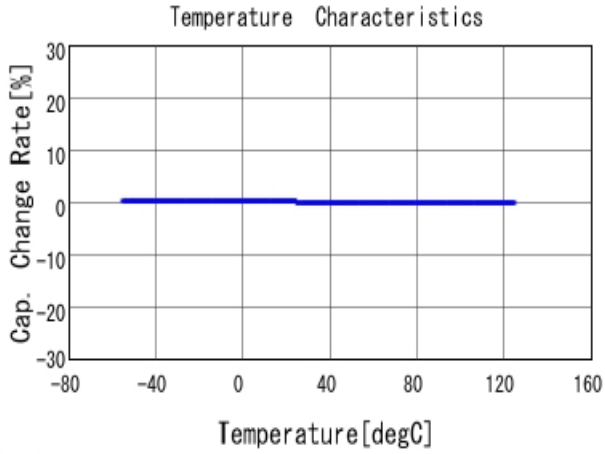
■ GRM2165C2A271JA01 C-Temp. capchange, DCOV, AC1Vrms
