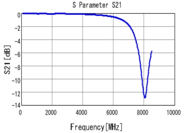
■ GRM2165C2A271JA01 S21 DCOV, 25degC
