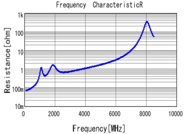
■ GRM2165C2A271JA01 R DCOV, 25degC
