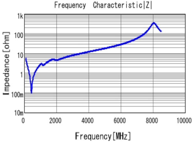
■ GRM2165C2A271JA01 |Z| DCOV, 25degC
