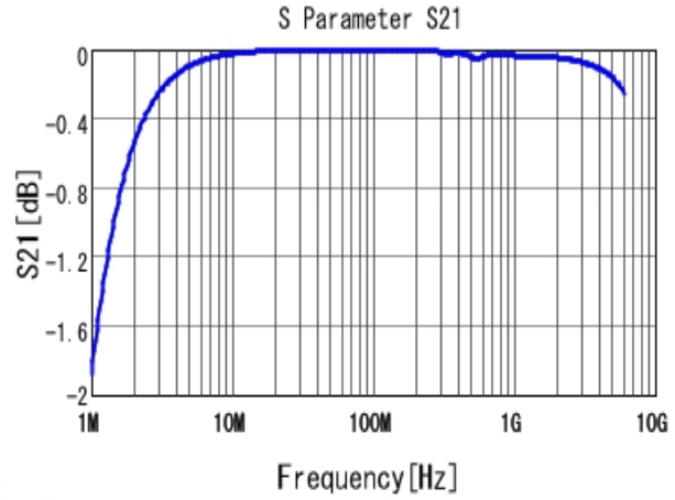
■ GRM2165C2A222JA01 S21 DCOV, 25degC
