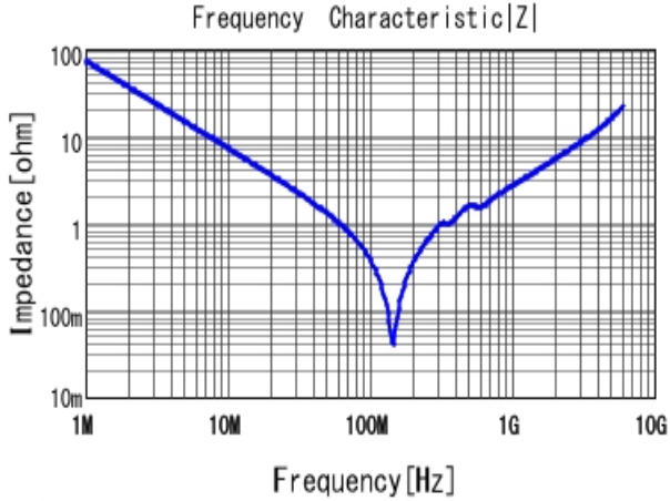
■ GRM2165C2A222JA01 |Z| DCOV, 25degC
