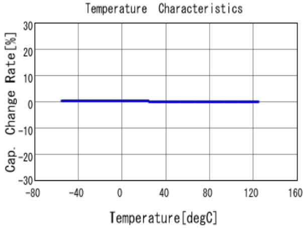
■ GRM2165C2A222JA01 C-Temp. capchange, DCOV, AC1Vrms
