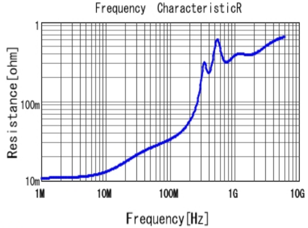
■ GRM2165C2A222JA01 R DCOV, 25degC
