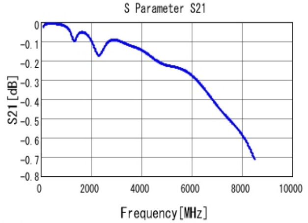
■ GRM2165C2A221JA01 S21 DCOV, 25degC
