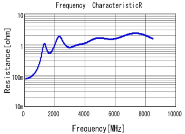
■ GRM2165C2A221JA01 R DCOV, 25degC
