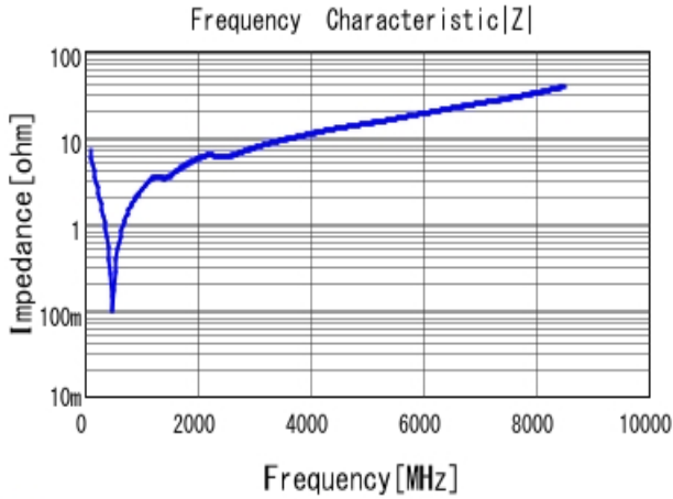
■ GRM2165C2A221JA01 |Z| DCOV, 25degC
