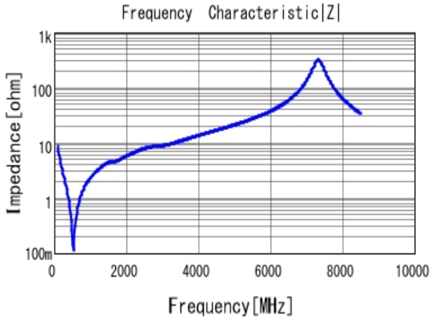
■ GRM2165C2A181JA01 |Z| DCOV, 25degC
