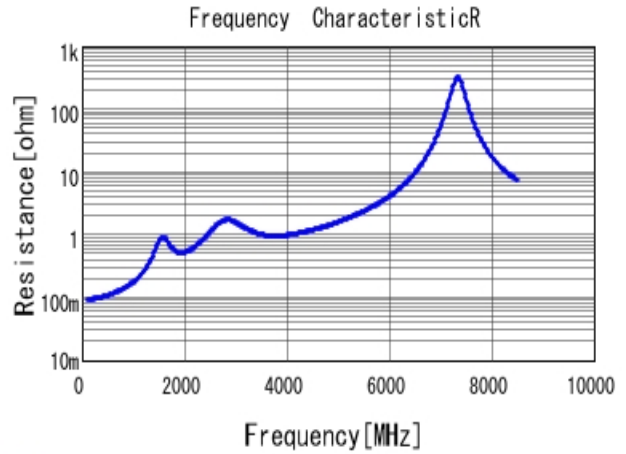
■ GRM2165C2A181JA01 R DCOV, 25degC
