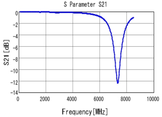
■ GRM2165C2A181JA01 S21 DCOV, 25degC
