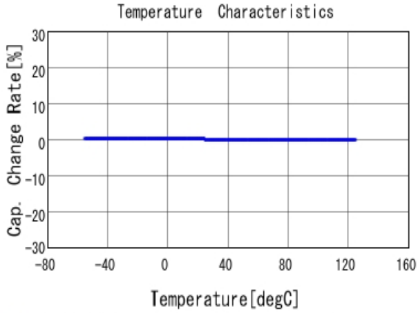
■ GRM2165C2A181JA01 C-Temp. capchange, DCOV, AC1Vrms
