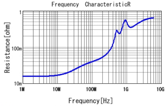
■ GRM2165C2A152JA01 R DCOV, 25degC
