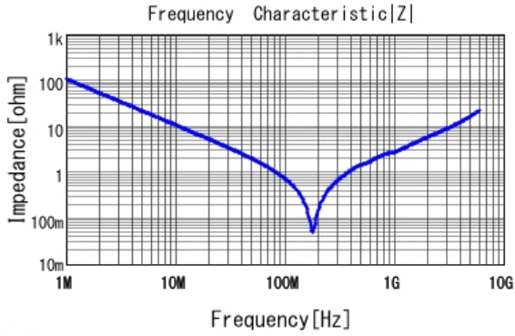
■ GRM2165C2A152JA01 |Z| DCOV, 25degC
