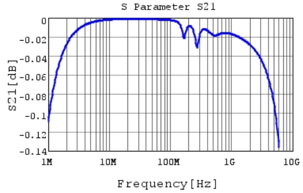
GRM2165C2A103JA01 S21 DCOV, 25degC
