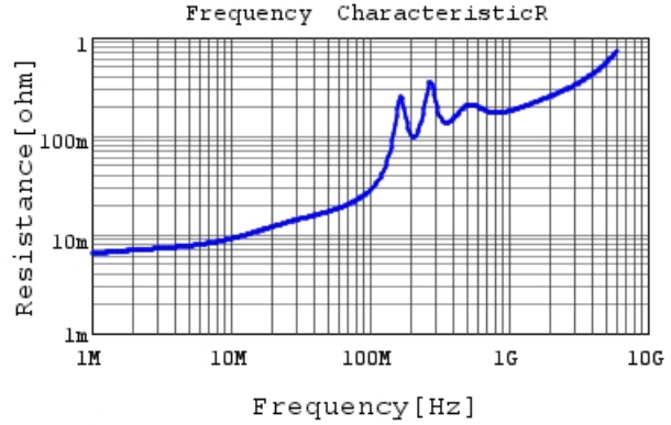
GRM2165C2A103JA01 R DCOV, 25degC
