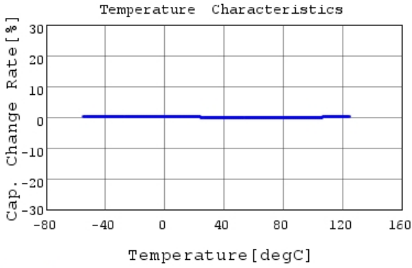
GRM2165C2A103JA01 C-Temp. capchange, DCOV, 1
