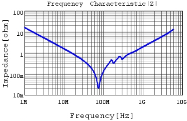
GRM2165C2A103JA01 |Z| DCOV, 25degC
